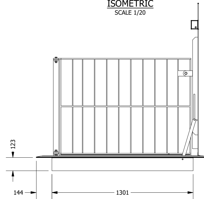
SIDE ELEVATION SCALE 1/20
