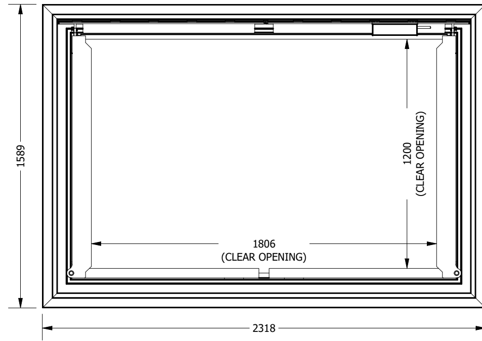
PLAN SCALE 1/20
