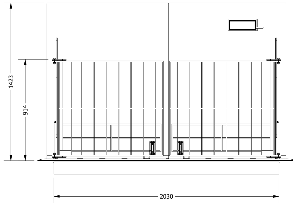
FRONT ELEVATION SCALE 1/20
