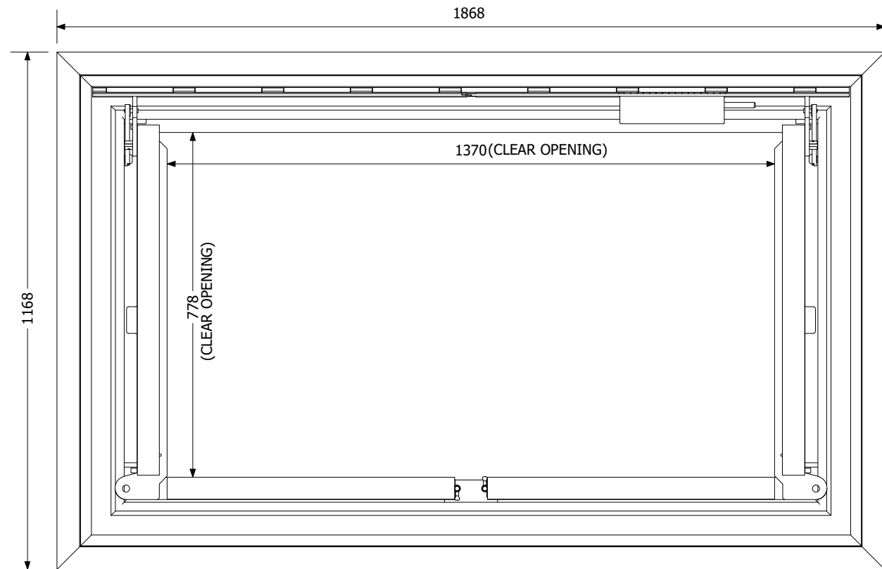
TOP VIEW NTS
