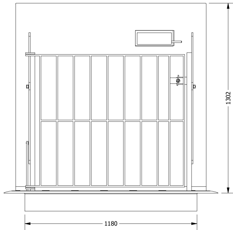
FRONT VIEW NTS
