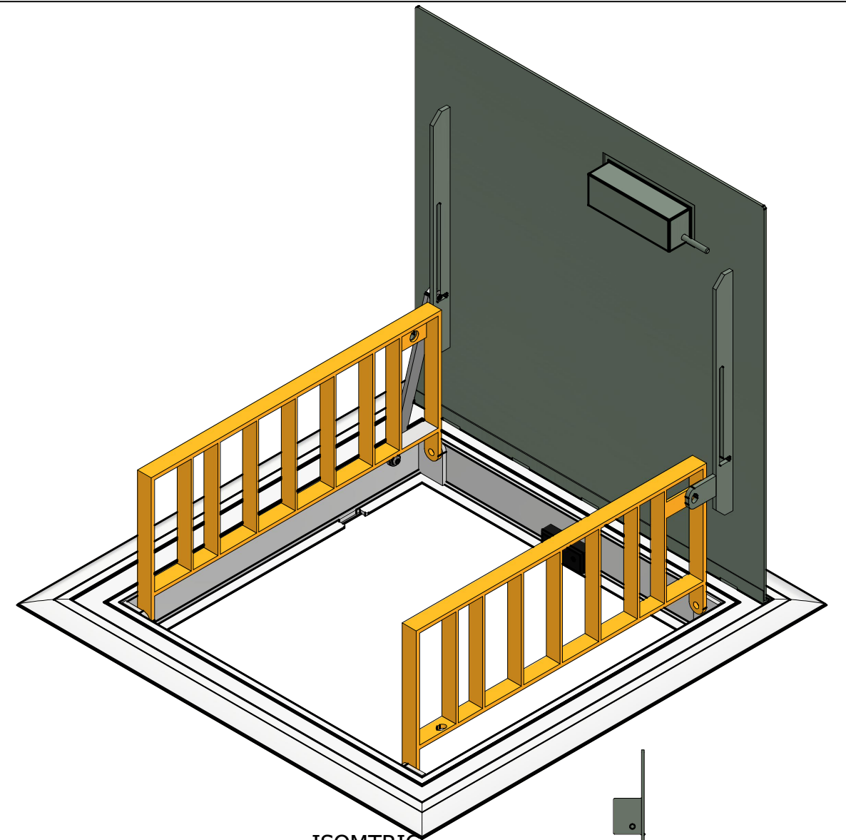
ISOMETRIC NTS
