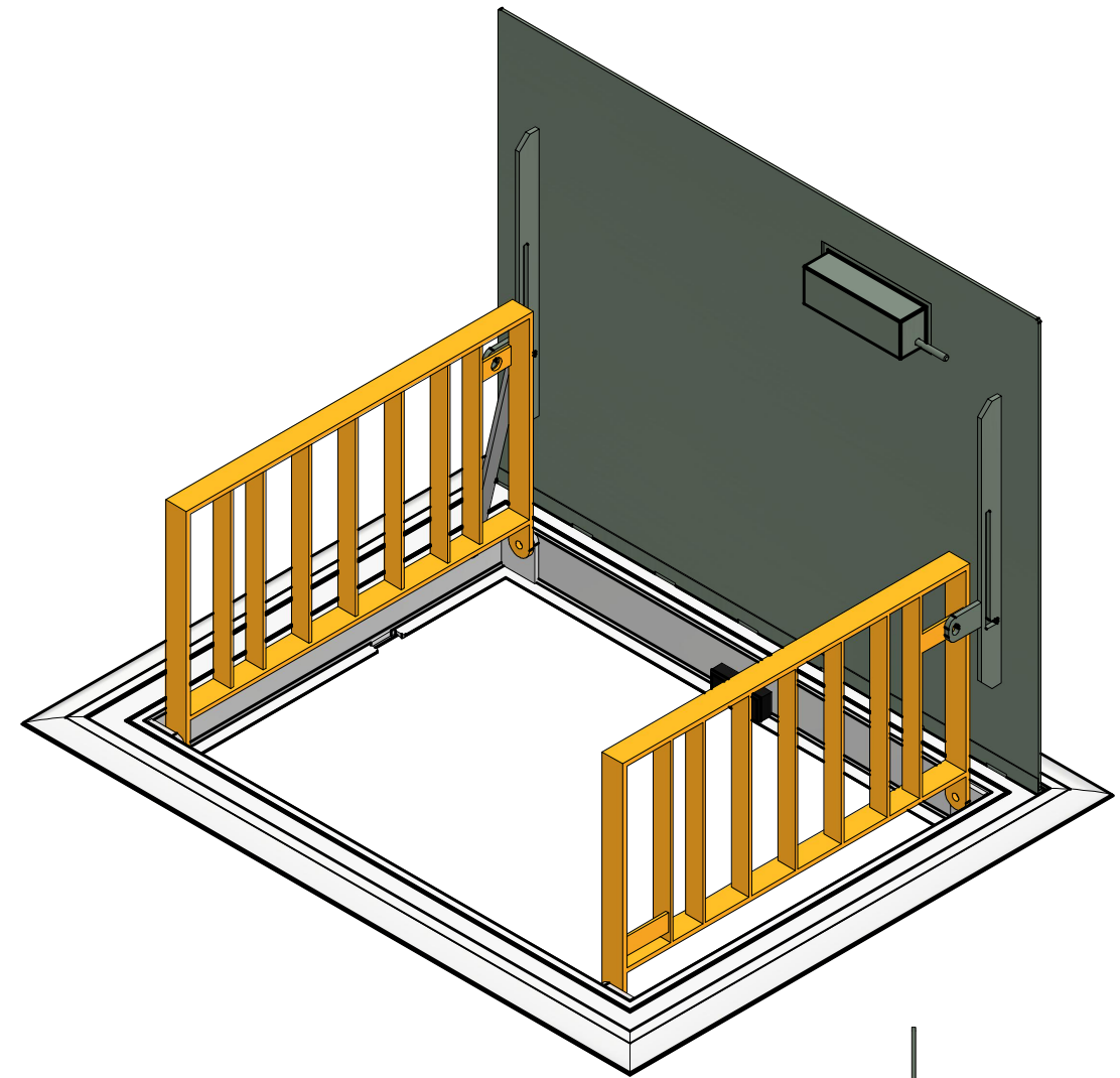
ISOMETRIC NTS
